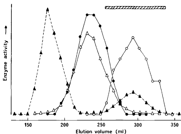
Fig. 1. Separation of galactosidases in extracts of T. foetus by chromatography on Sephadex G-200. (○) Blood-group P 1 -destroying enzyme ( \alpha -galactosidase a ); (●) blood-group B-destroying enzyme ( \alpha -galactosidase b ); (△), p -nitrophenyl \alpha -D-galactoside hydrolysing enzyme ( \alpha -galactosidase c ); (▲) p -nitrophenyl \beta -D-galactoside hydrolysing enzyme ( \beta -galactosidase); (hatched area) Fractions pooled for isoelectric focusing.
