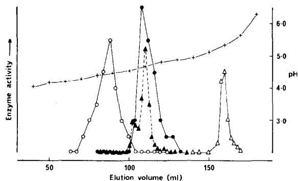
Fig. 2. Separation by isoelectric focusing of galactosidases in pooled blood-group P 1 -destroying enzyme fractions from Sephadex G-200 column (fig. 1). (+) pH gradient; other symbols as in (fig. 1).
